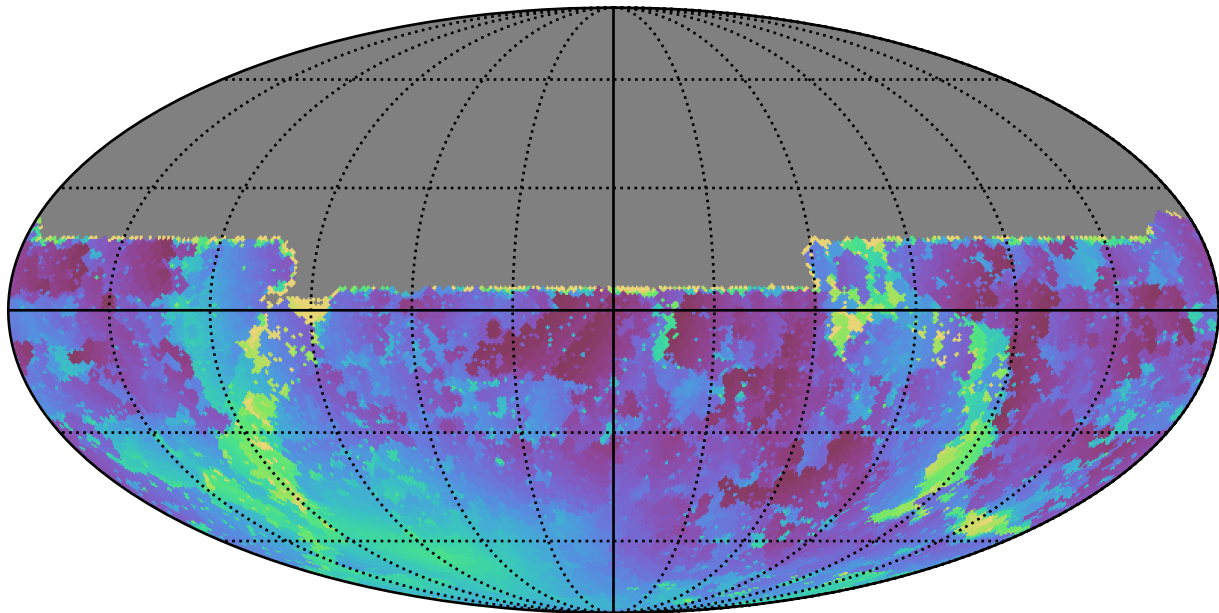
all_long_v3.4_10yrs All sky u band: Min moonDistance
