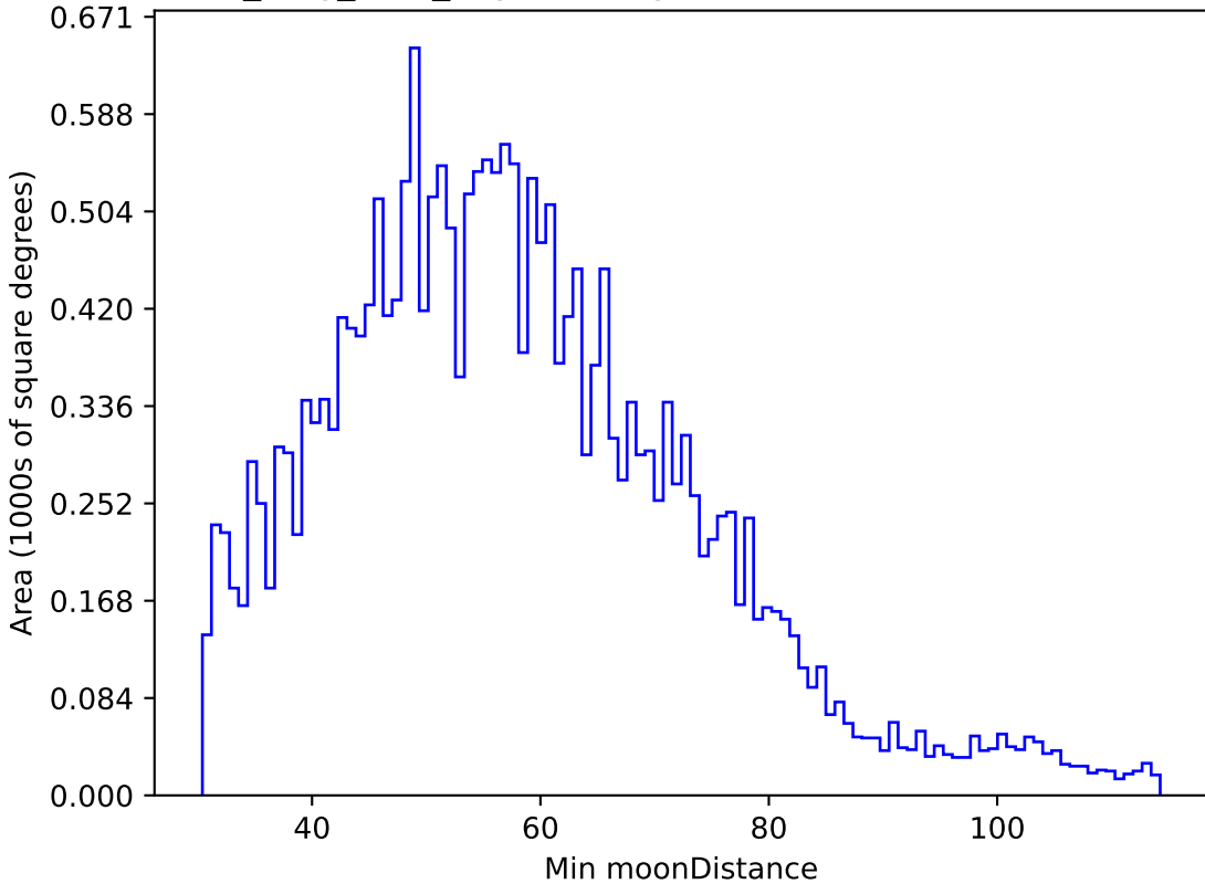
all_long_v3.4_10yrs All sky u band: Min moonDistance
