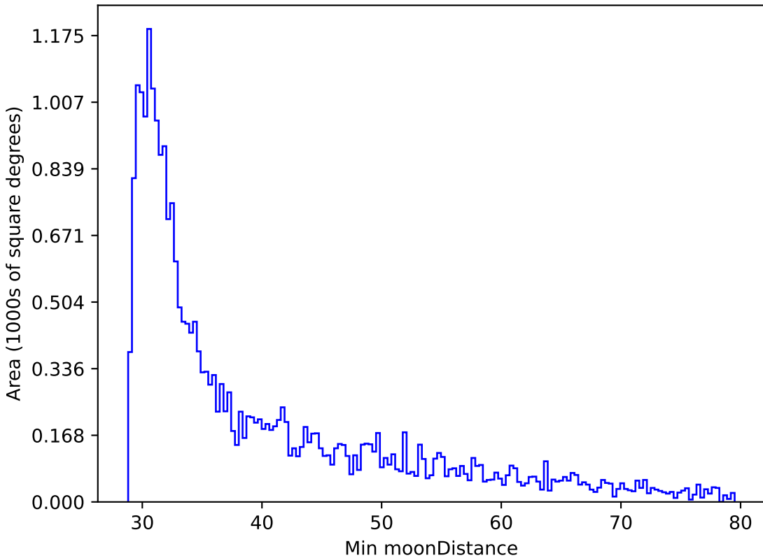
all_long_v3.4_10yrs All sky r band: Min moonDistance
