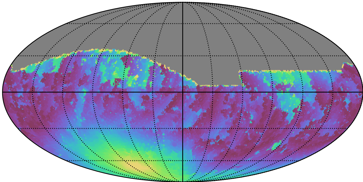
all_long_v3.4_10yrs All sky g band: Min moonDistance
