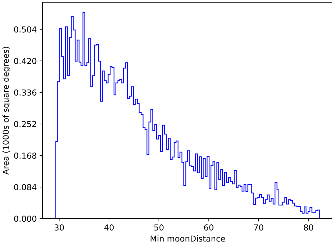
all_long_v3.4_10yrs All sky g band: Min moonDistance
