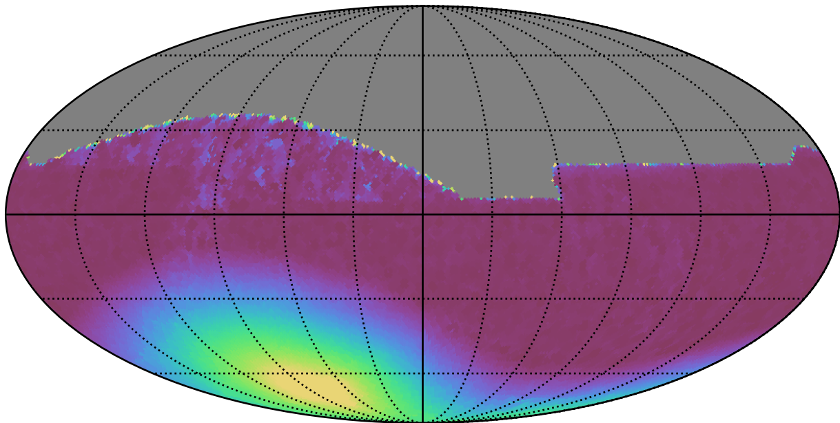
all_long_v3.4_10yrs All sky all bands: Min moonDistance
