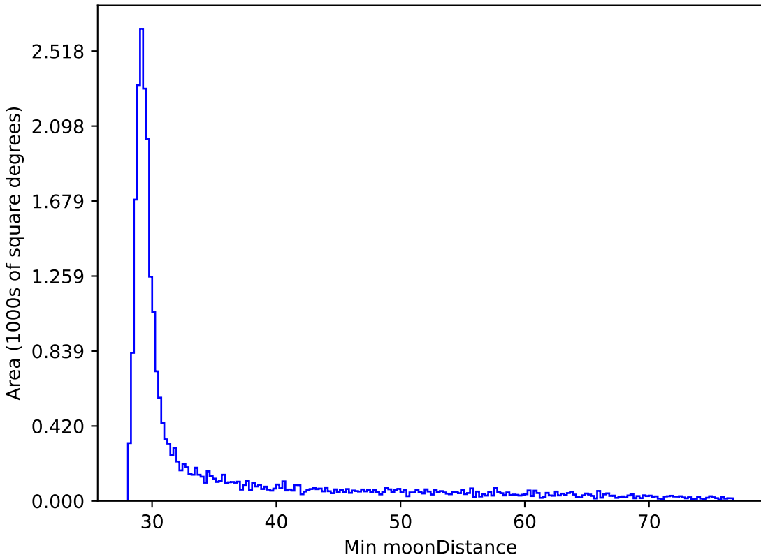
all_long_v3.4_10yrs All sky all bands: Min moonDistance
