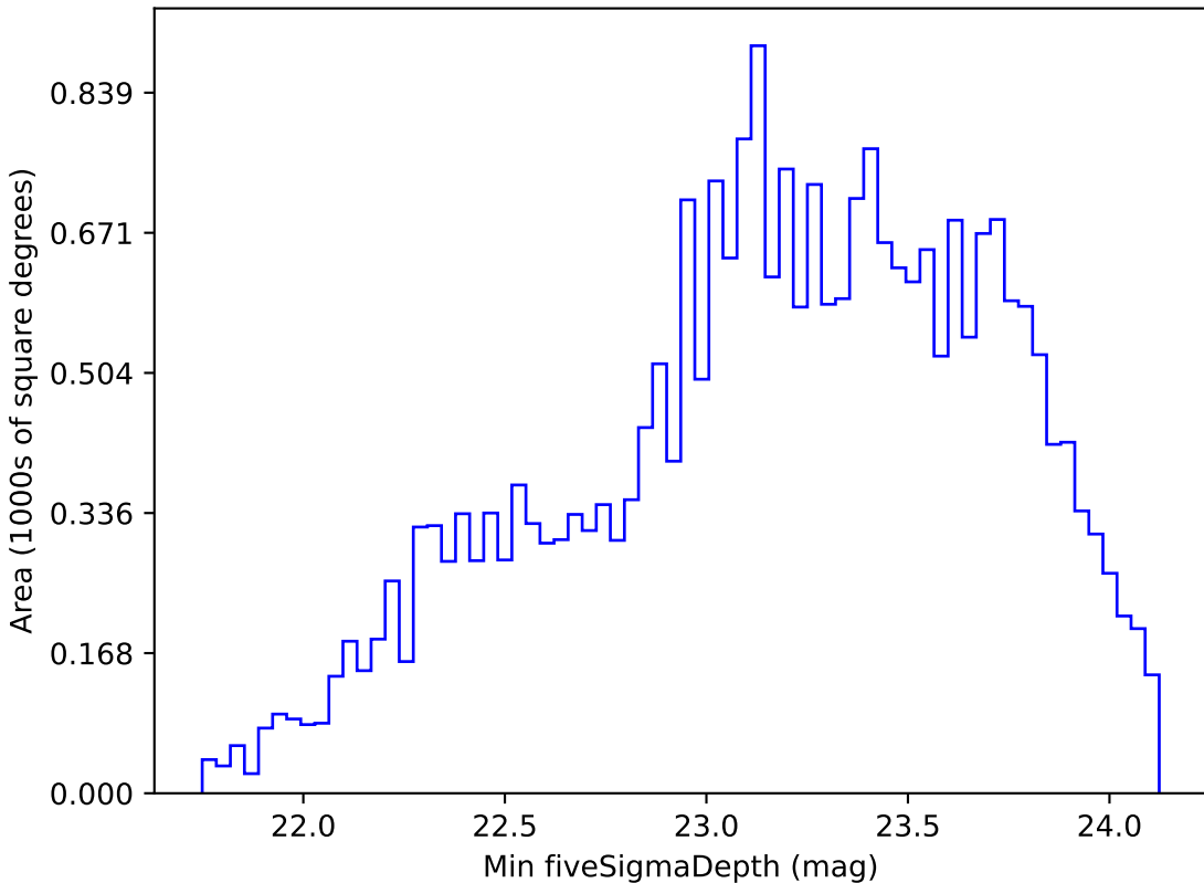
all_long_v3.4_10yrs Yr 1 r band: Min fiveSigmaDepth
