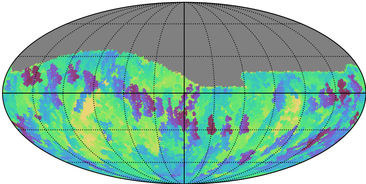
all_long_v3.4_10yrs Yr 1 i band: Min fiveSigmaDepth
