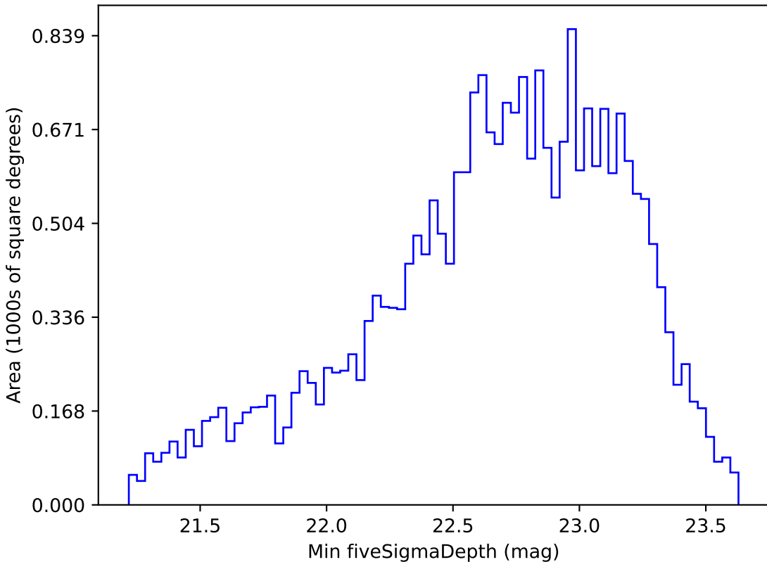
all_long_v3.4_10yrs Yr 1 i band: Min fiveSigmaDepth
