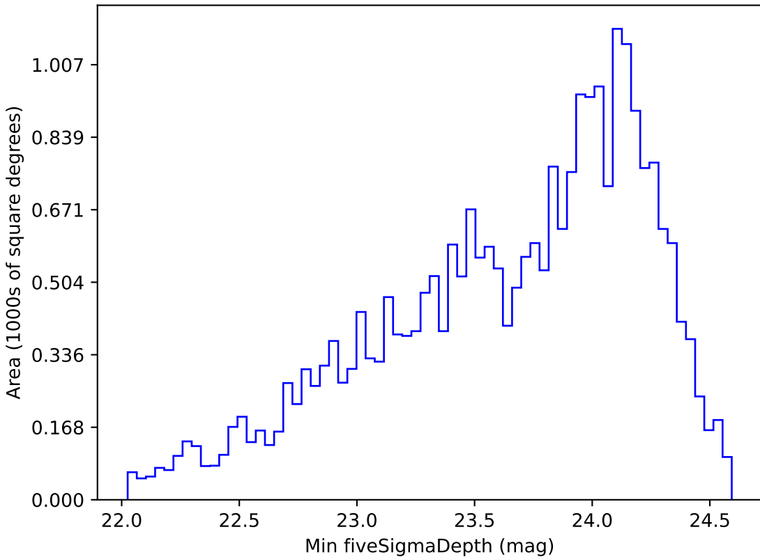
all_long_v3.4_10yrs Yr 1 g band: Min fiveSigmaDepth
