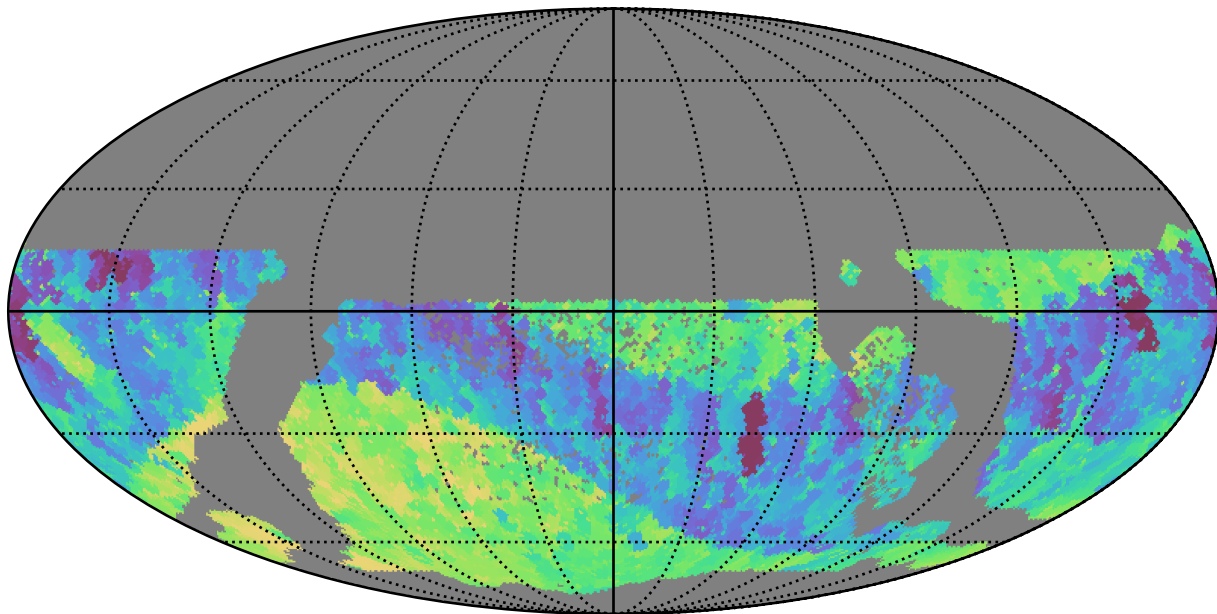
all_long_v3.4_10yrs WFD z band: Min fiveSigmaDepth
