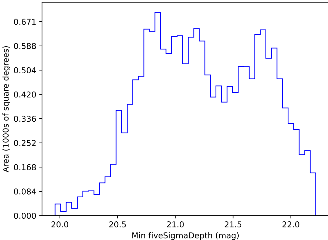
all_long_v3.4_10yrs WFD z band: Min fiveSigmaDepth
