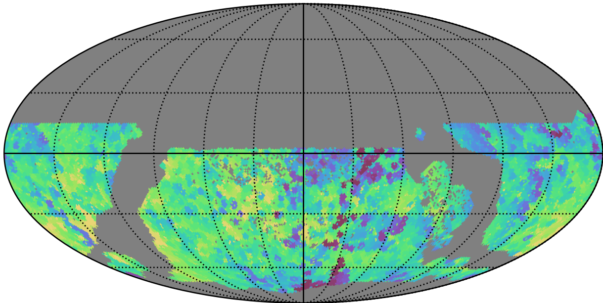
all_long_v3.4_10yrs WFD y band: Min fiveSigmaDepth
