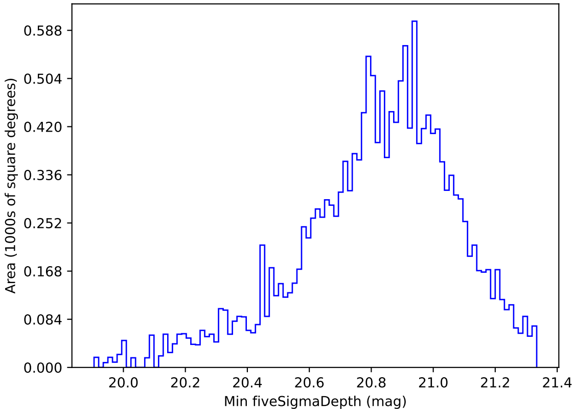
all_long_v3.4_10yrs WFD y band: Min fiveSigmaDepth
