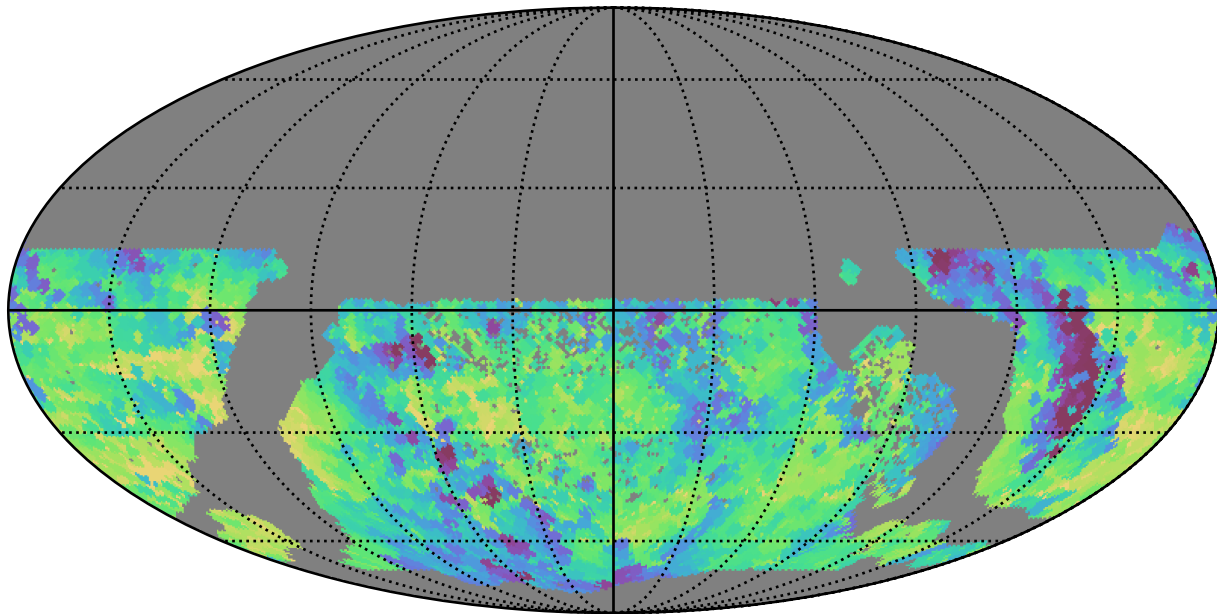
all_long_v3.4_10yrs WFD u band: Min fiveSigmaDepth
