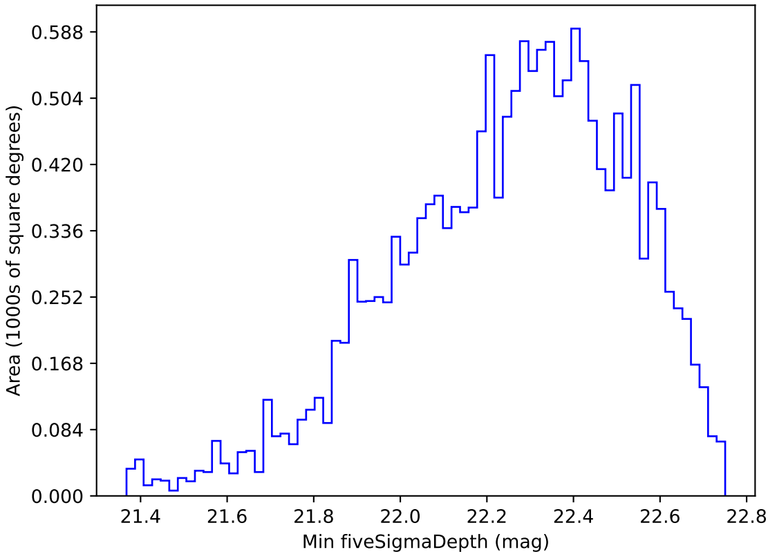
all_long_v3.4_10yrs WFD u band: Min fiveSigmaDepth
