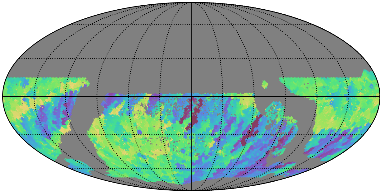
all_long_v3.4_10yrs WFD r band: Min fiveSigmaDepth
