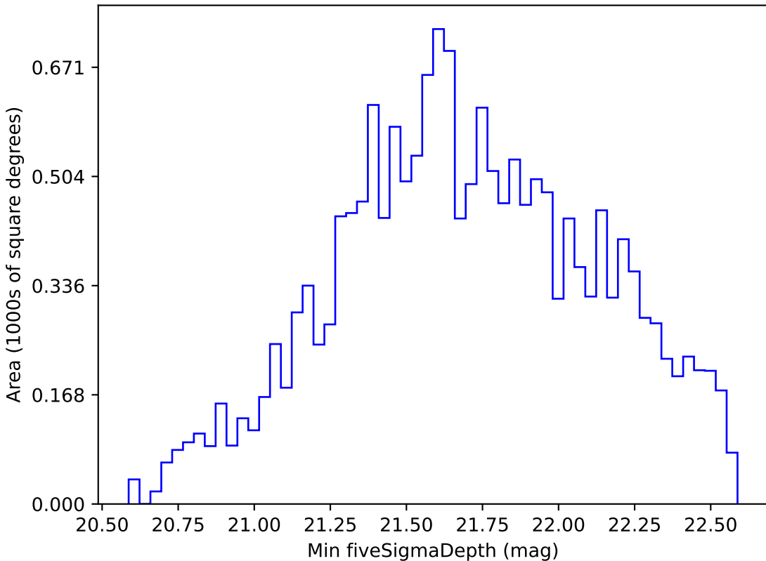
all_long_v3.4_10yrs WFD i band: Min fiveSigmaDepth
