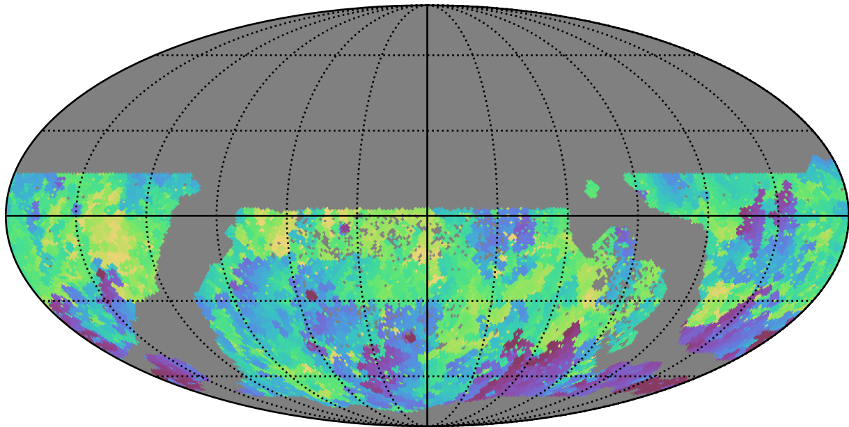
all_long_v3.4_10yrs WFD g band: Min fiveSigmaDepth
