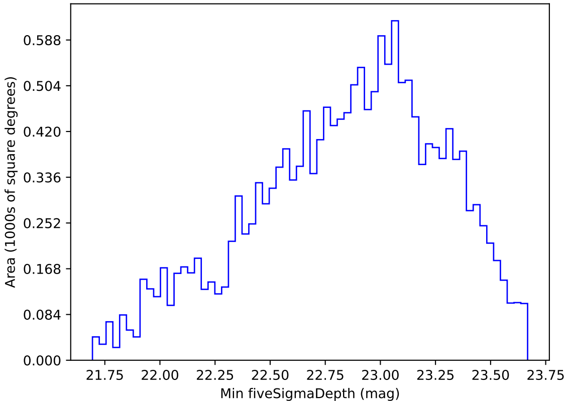
all_long_v3.4_10yrs WFD g band: Min fiveSigmaDepth
