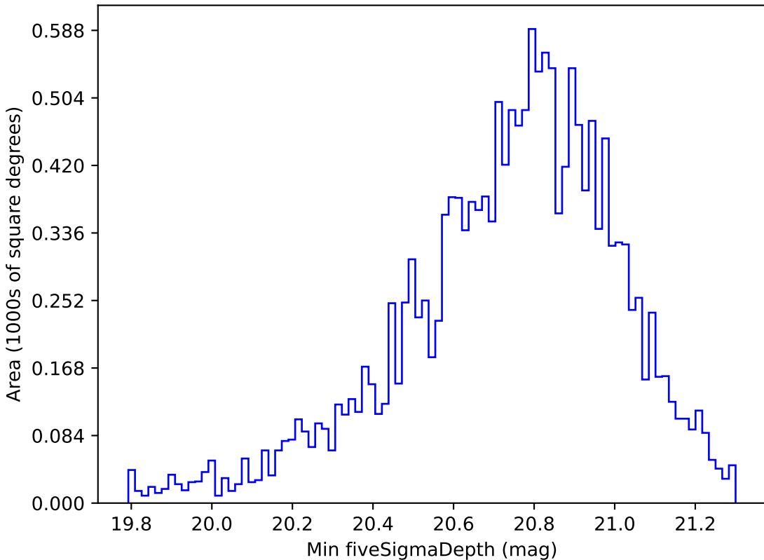
all_long_v3.4_10yrs WFD all bands: Min fiveSigmaDepth
