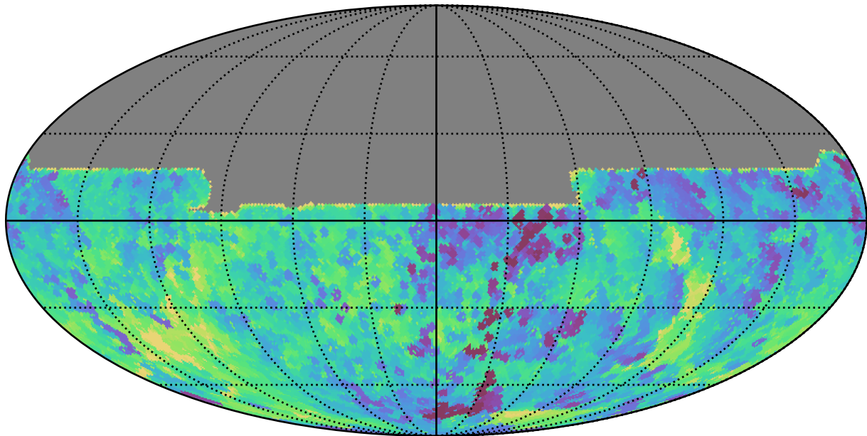
all_long_v3.4_10yrs All sky y band: Min fiveSigmaDepth
