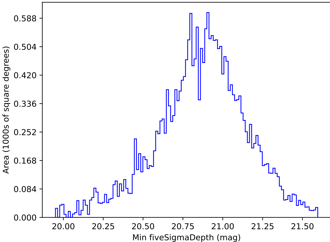
all_long_v3.4_10yrs All sky y band: Min fiveSigmaDepth
