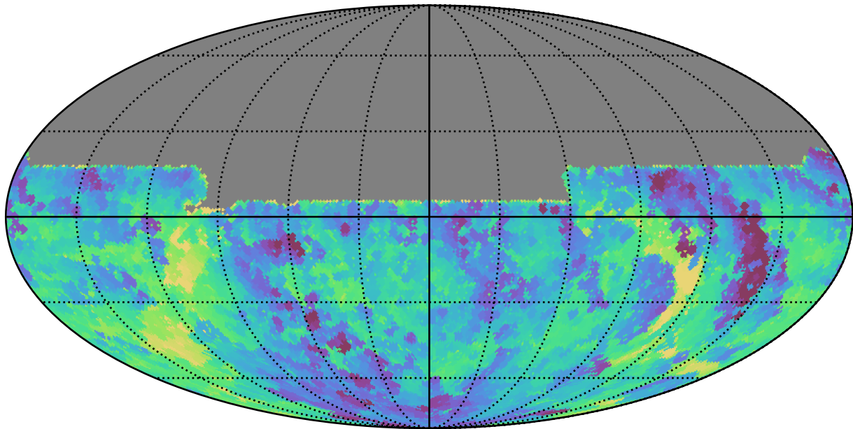
all_long_v3.4_10yrs All sky u band: Min fiveSigmaDepth
