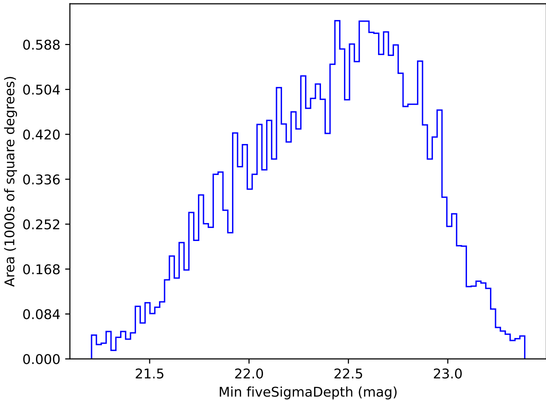
all_long_v3.4_10yrs All sky r band: Min fiveSigmaDepth
