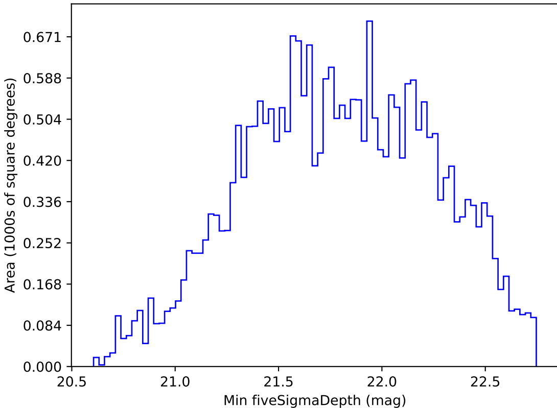
all_long_v3.4_10yrs All sky i band: Min fiveSigmaDepth
