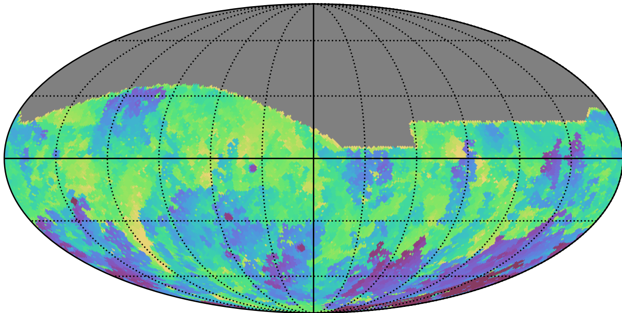
all_long_v3.4_10yrs All sky g band: Min fiveSigmaDepth
