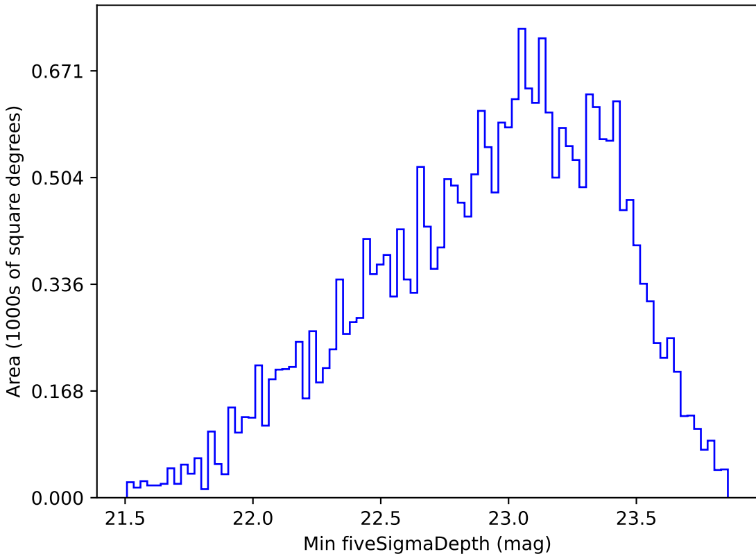
all_long_v3.4_10yrs All sky g band: Min fiveSigmaDepth
