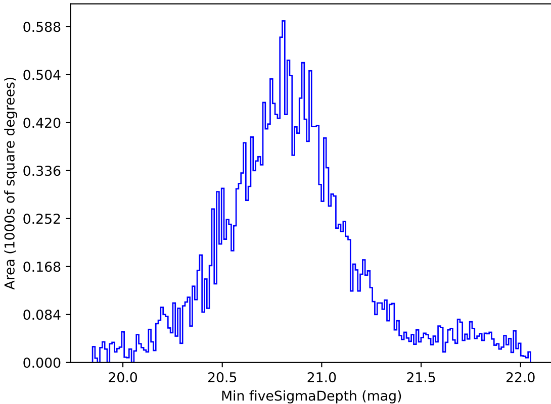
all_long_v3.4_10yrs All sky all bands: Min fiveSigmaDepth
