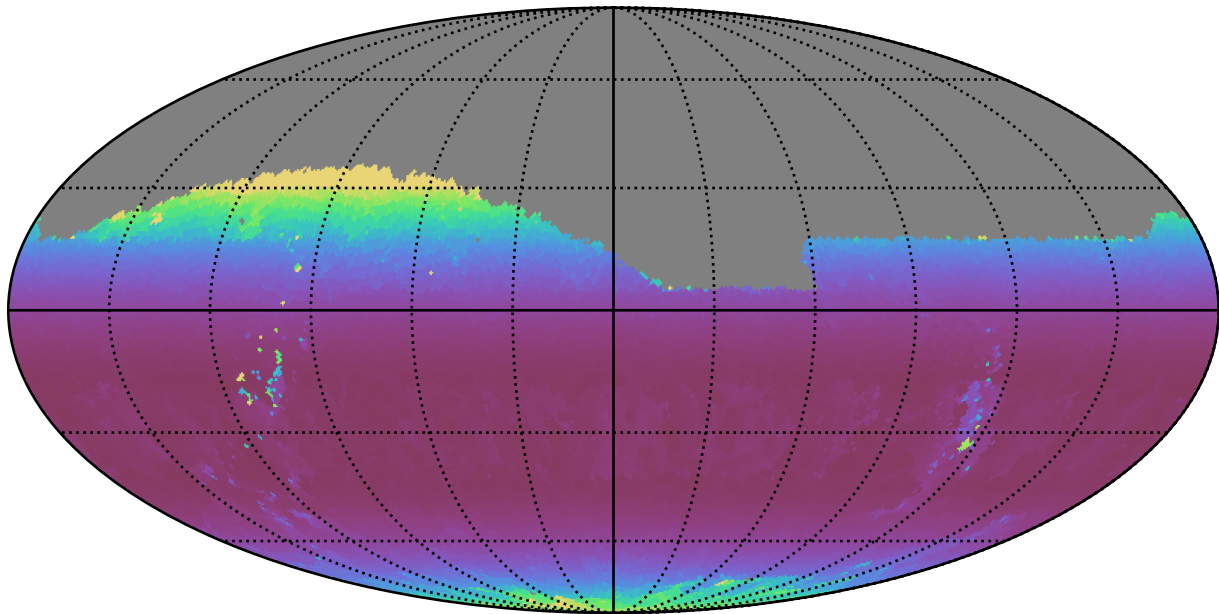
all_long_v3.4_10yrs Yr 1 z band: Min airmass
