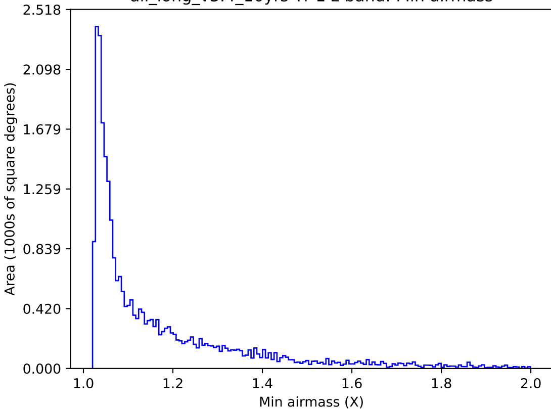
all_long_v3.4_10yrs Yr 1 z band: Min airmass
