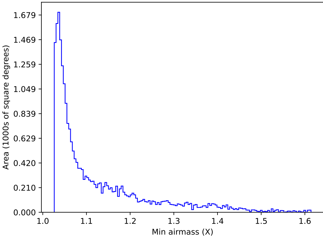
all_long_v3.4_10yrs Yr 1 y band: Min airmass
