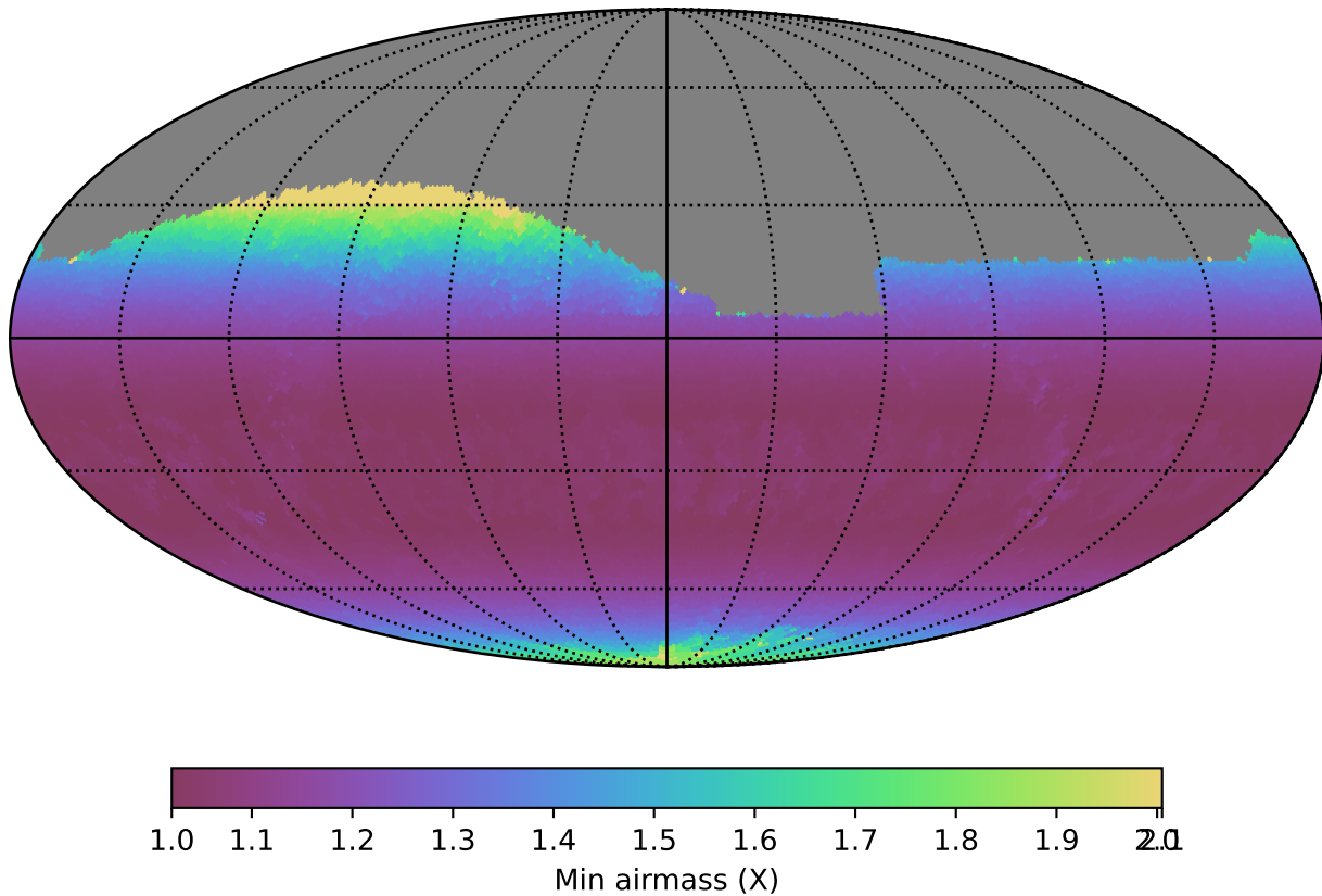
all_long_v3.4_10yrs Yr 1 r band: Min airmass
