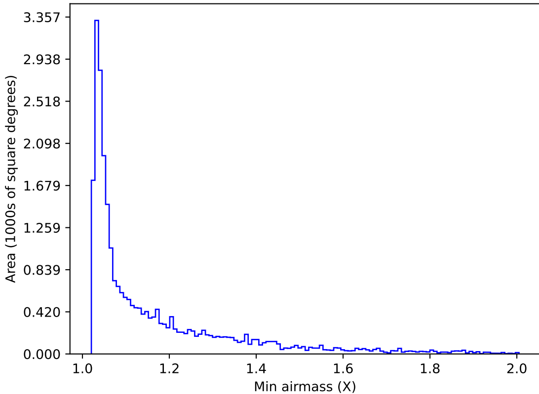
all_long_v3.4_10yrs Yr 1 r band: Min airmass
