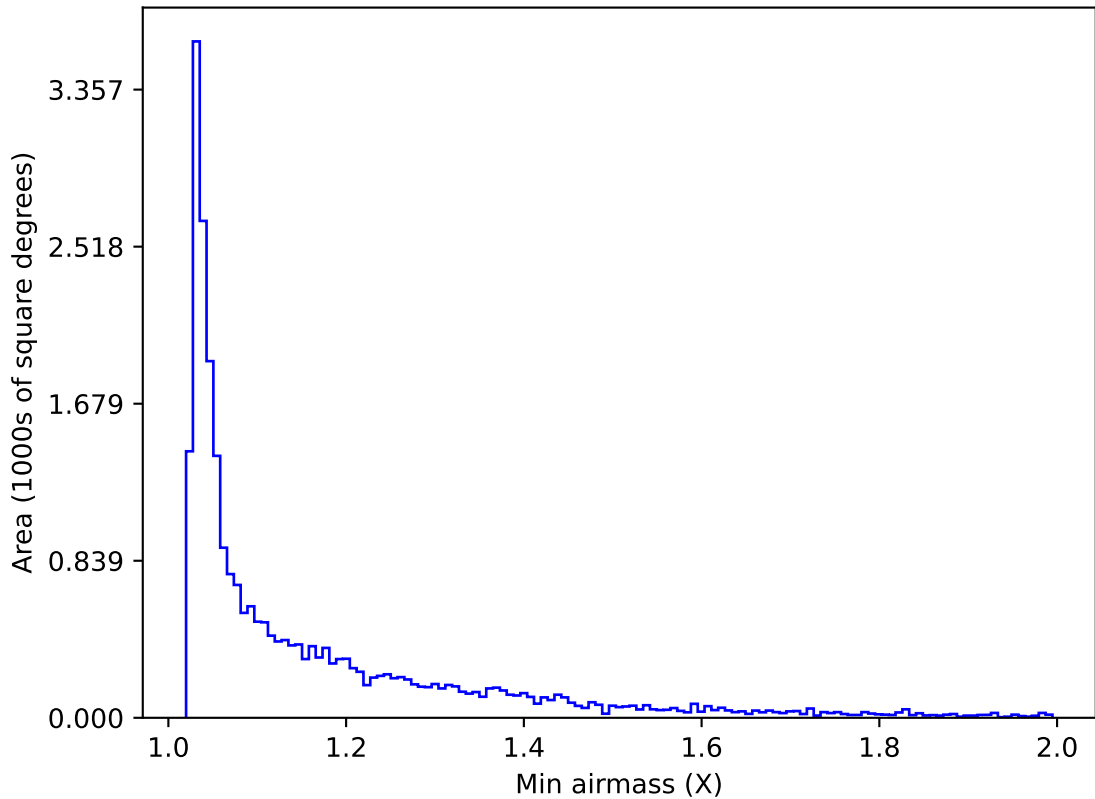
all_long_v3.4_10yrs Yr 1 i band: Min airmass
