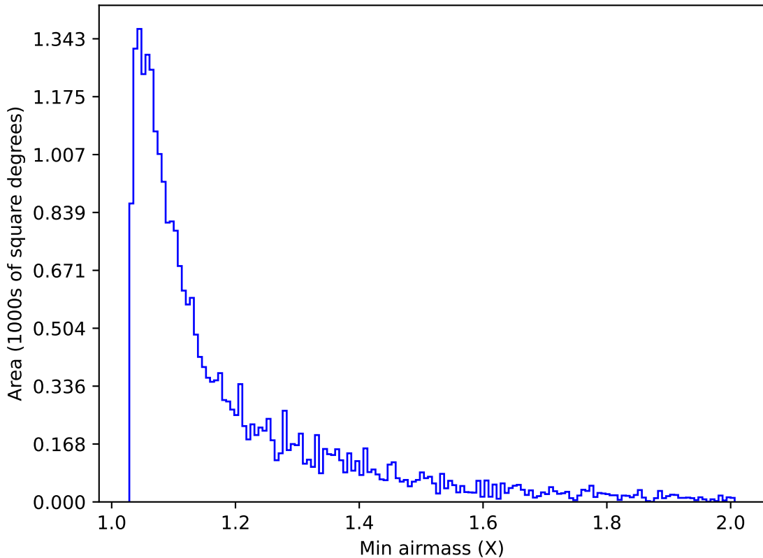
all_long_v3.4_10yrs Yr 1 g band: Min airmass
