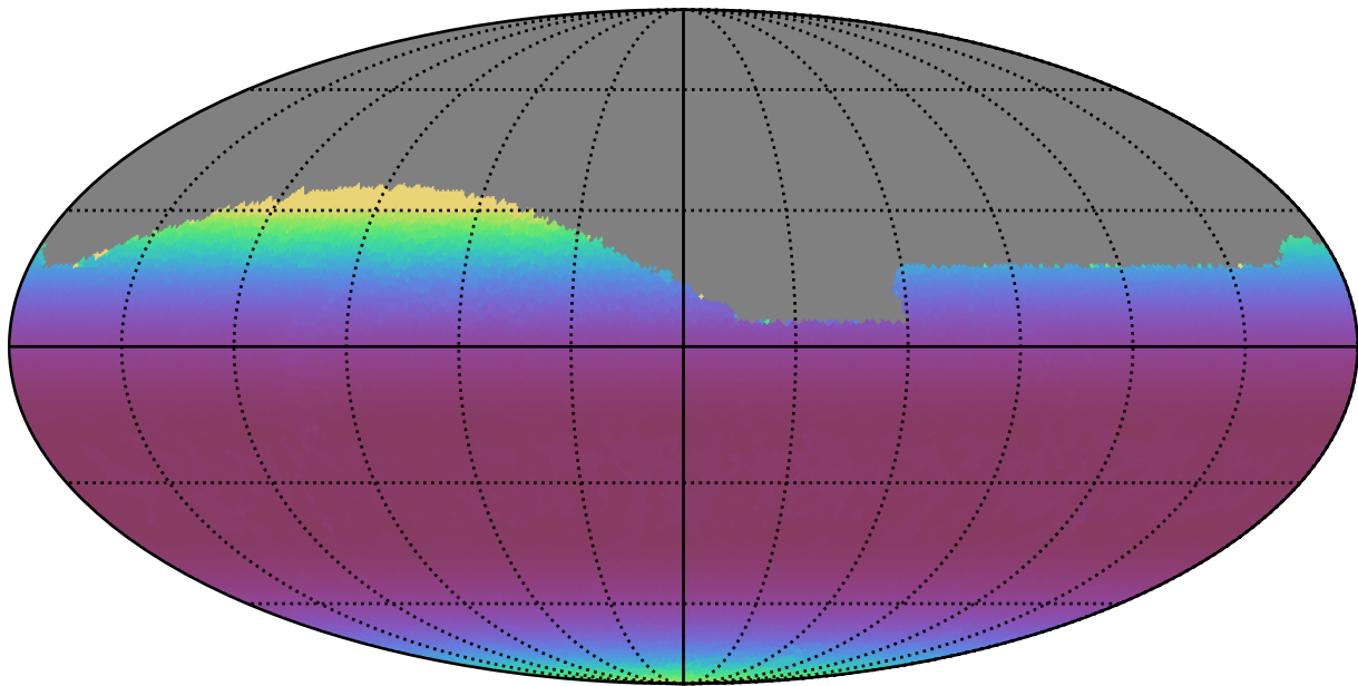
all_long_v3.4_10yrs Yr 1 all bands: Min airmass
