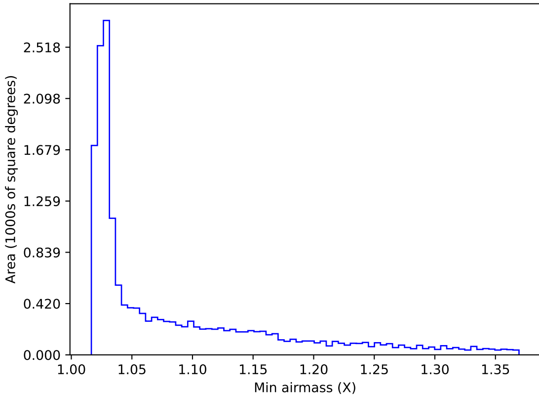
all_long_v3.4_10yrs WFD z band: Min airmass
