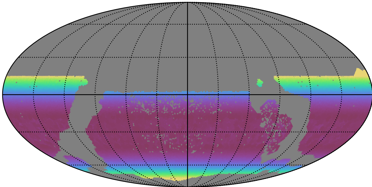
all_long_v3.4_10yrs WFD y band: Min airmass
