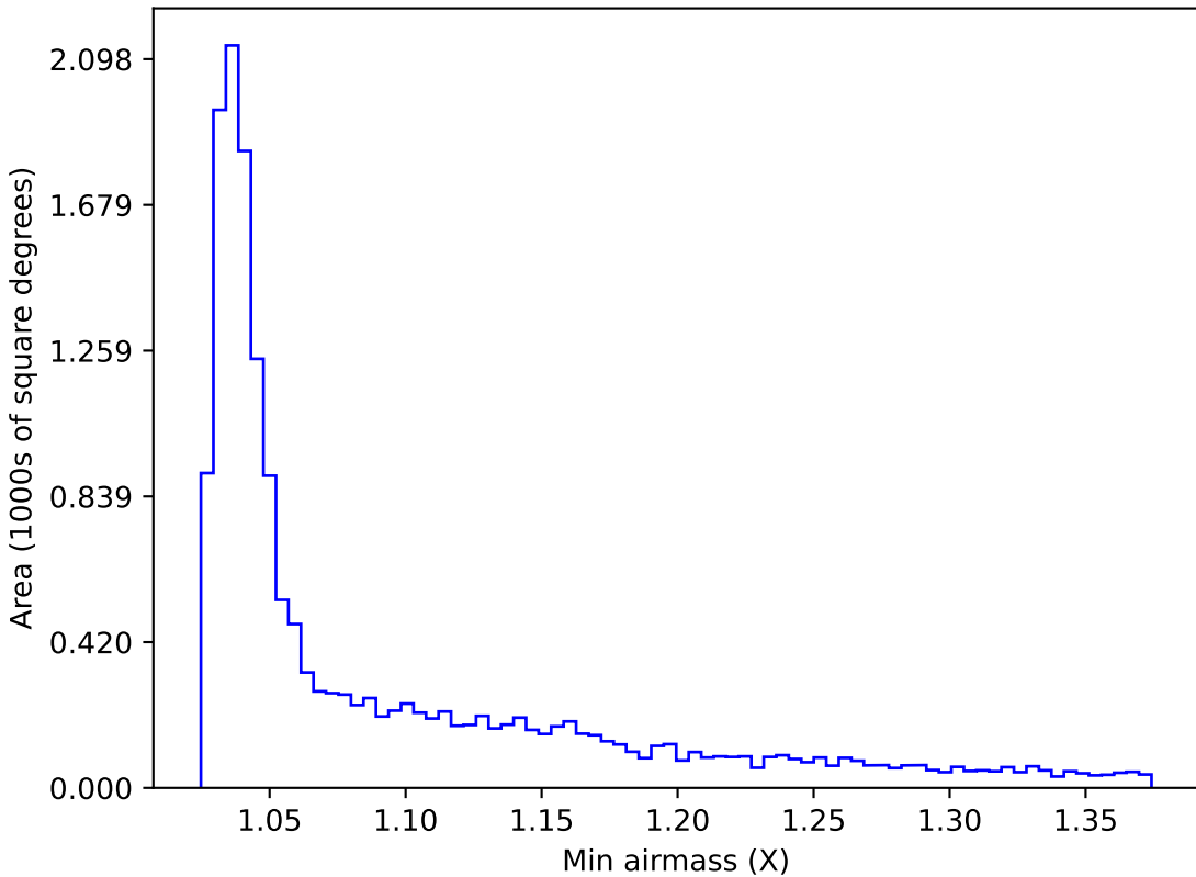
all_long_v3.4_10yrs WFD u band: Min airmass
