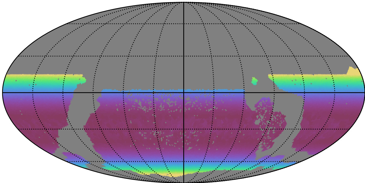
all_long_v3.4_10yrs WFD r band: Min airmass
