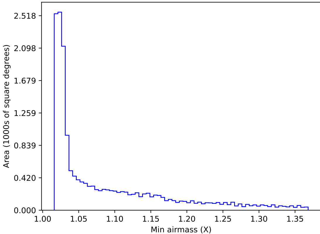
all_long_v3.4_10yrs WFD r band: Min airmass
