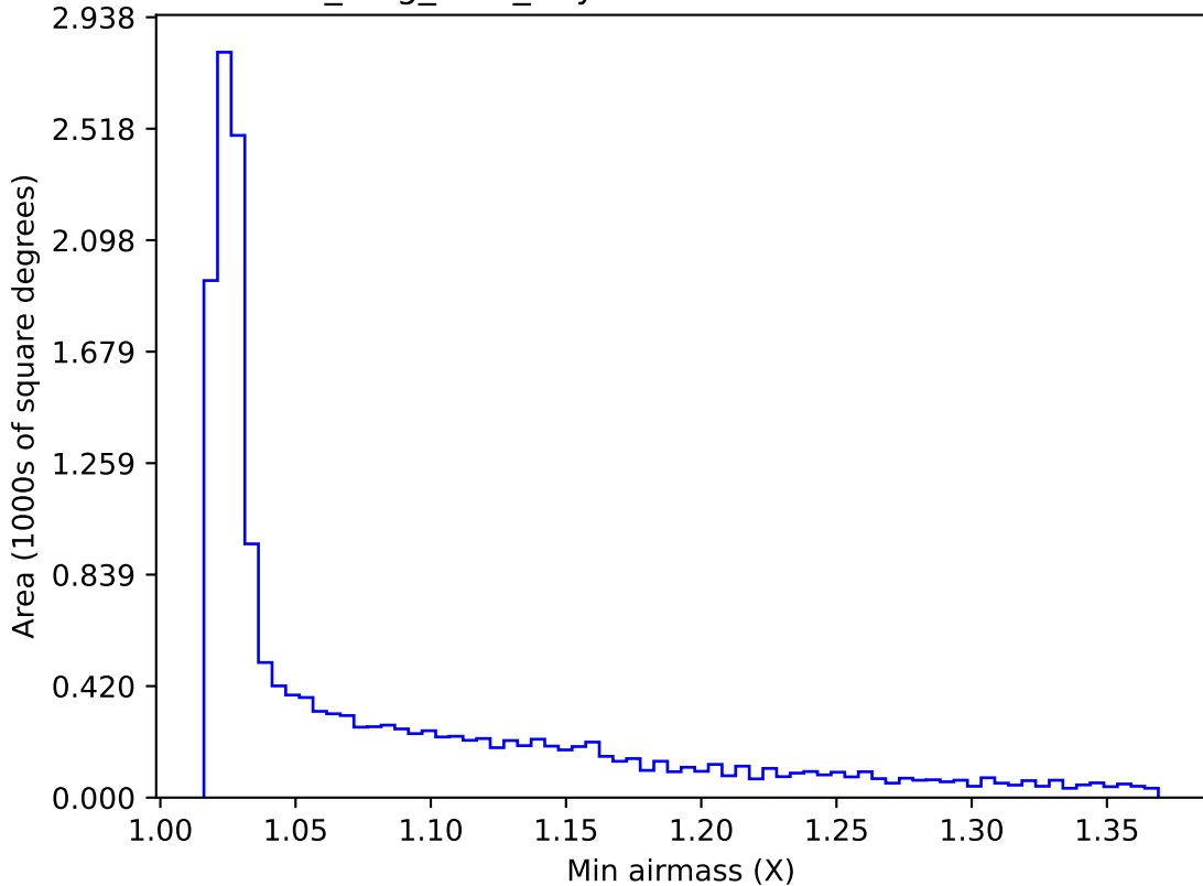
all_long_v3.4_10yrs WFD i band: Min airmass
