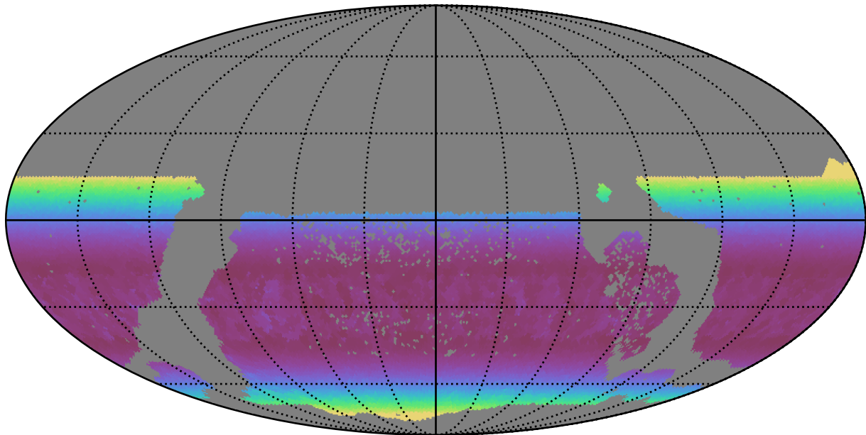
all_long_v3.4_10yrs WFD g band: Min airmass
