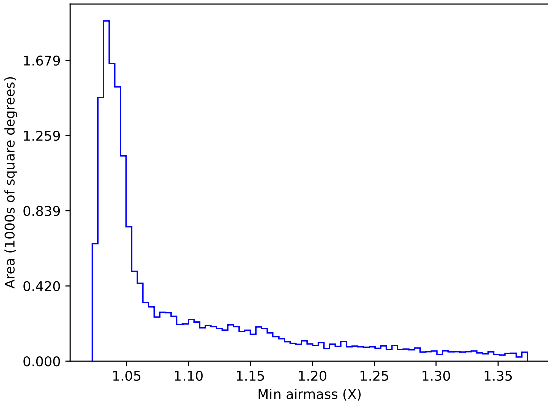
all_long_v3.4_10yrs WFD g band: Min airmass
