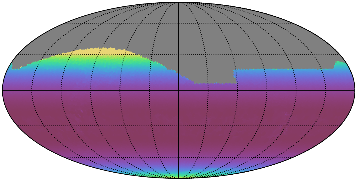
all_long_v3.4_10yrs All sky z band: Min airmass
