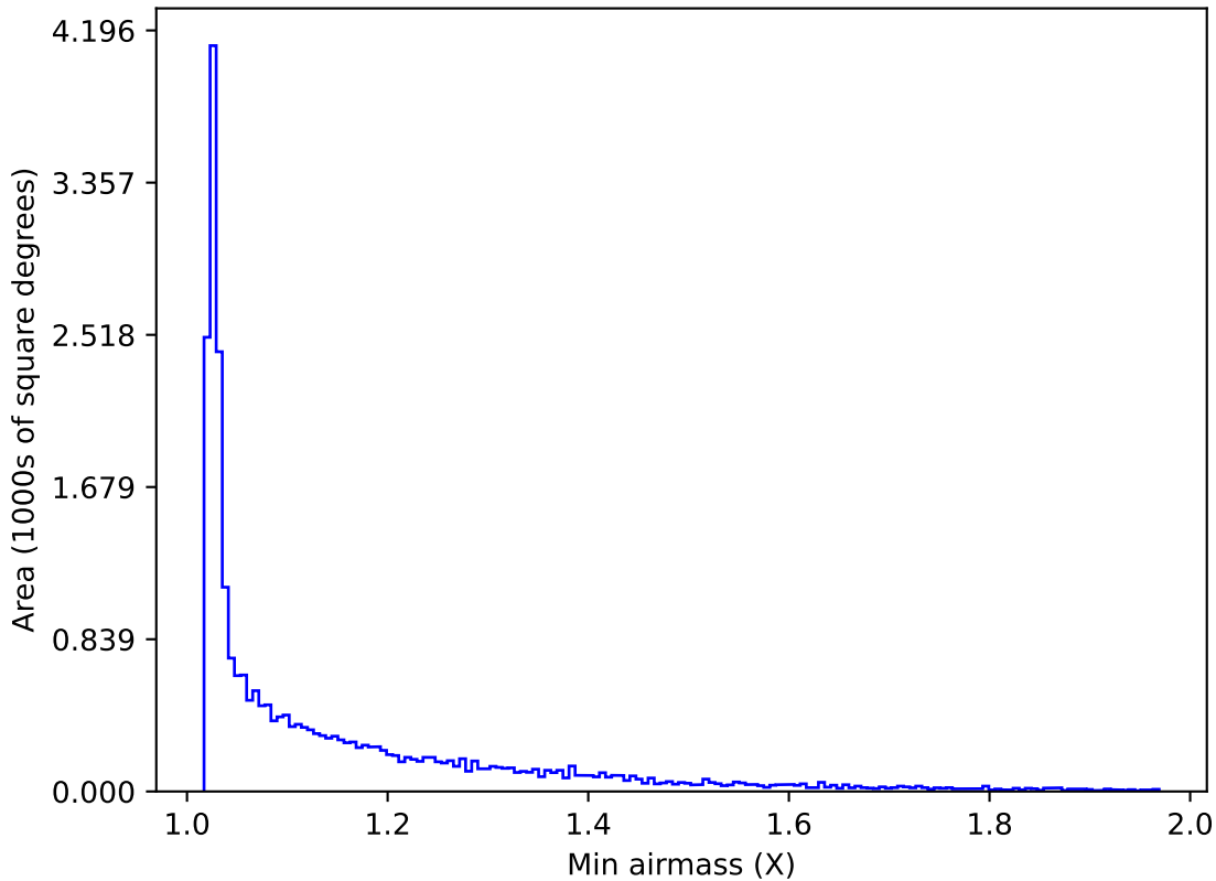
all_long_v3.4_10yrs All sky z band: Min airmass
