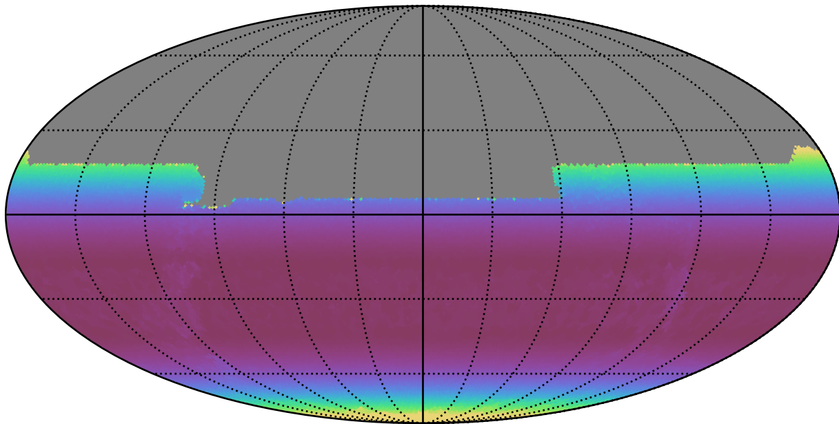
all_long_v3.4_10yrs All sky y band: Min airmass
