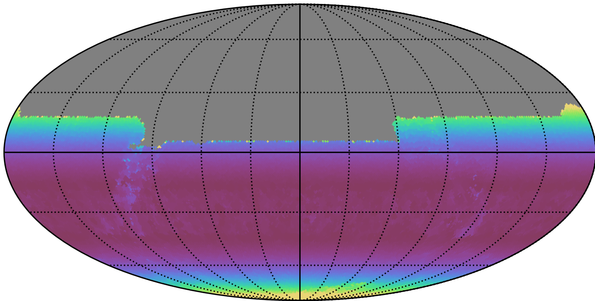
all_long_v3.4_10yrs All sky u band: Min airmass
